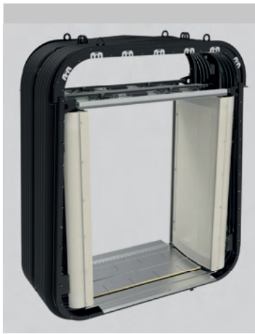
Metro gangway with flexible sidewall panels
