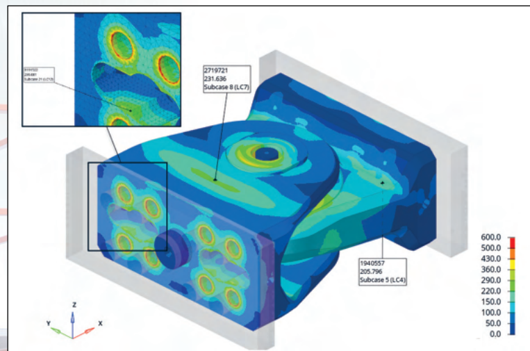
Strength verified by FEM calculations
